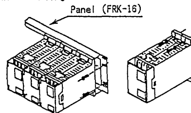
Fig.2 Wall Mounting
